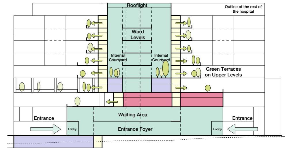
A cross section through the middle of the new hospital.
